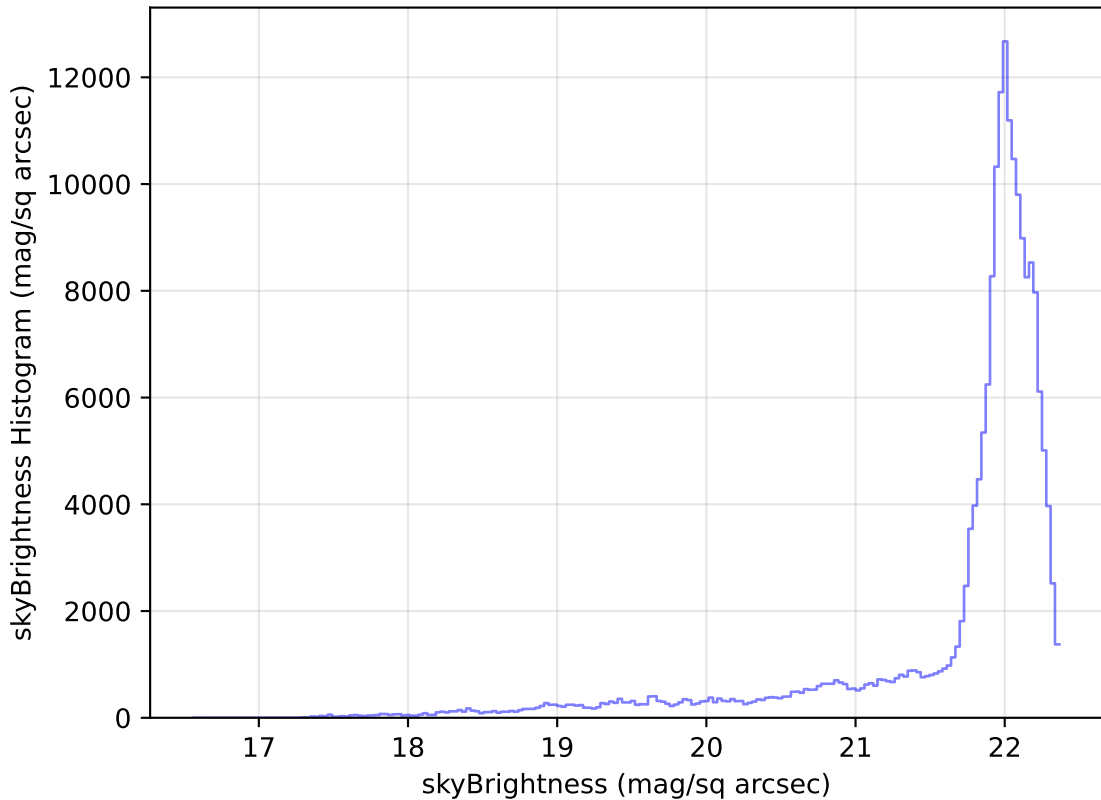
too_elab_r256_d2_gz_v3.4_10yrs WFD g band: skyBrightness Histogram
