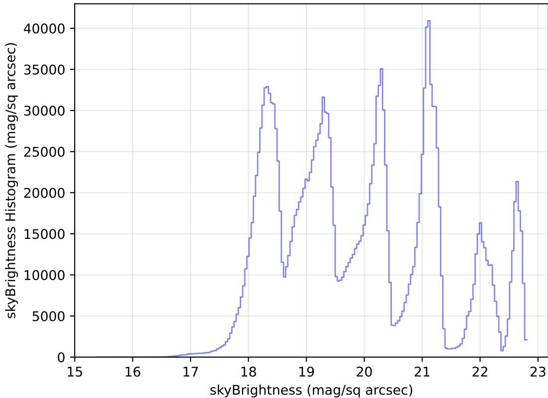
too_elab_r256_d2_gz_v3.4_10yrs WFD all bands: skyBrightness Histogram
