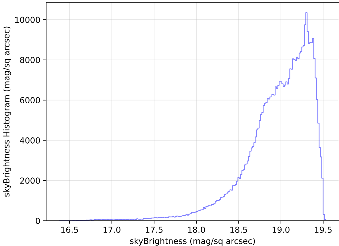
too_elab_r256_d2_gz_v3.4_10yrs All sky z band: skyBrightness Histogram
