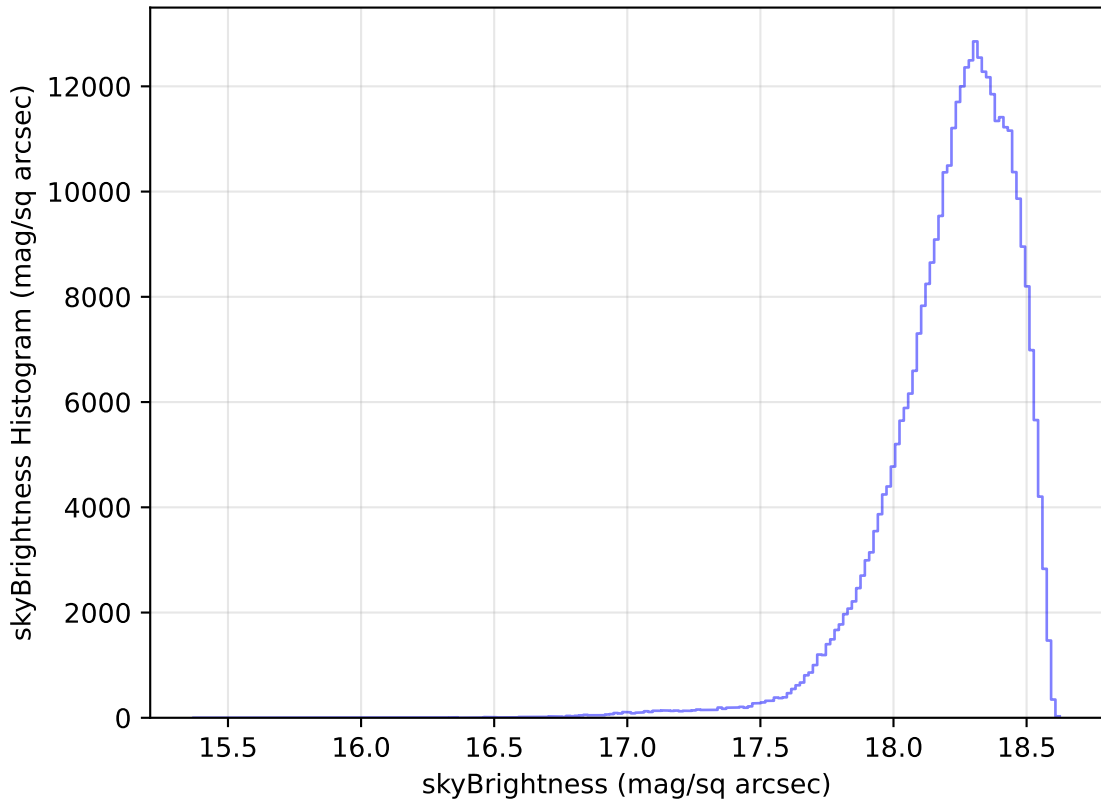
too_elab_r256_d2_gz_v3.4_10yrs All sky y band: skyBrightness Histogram
