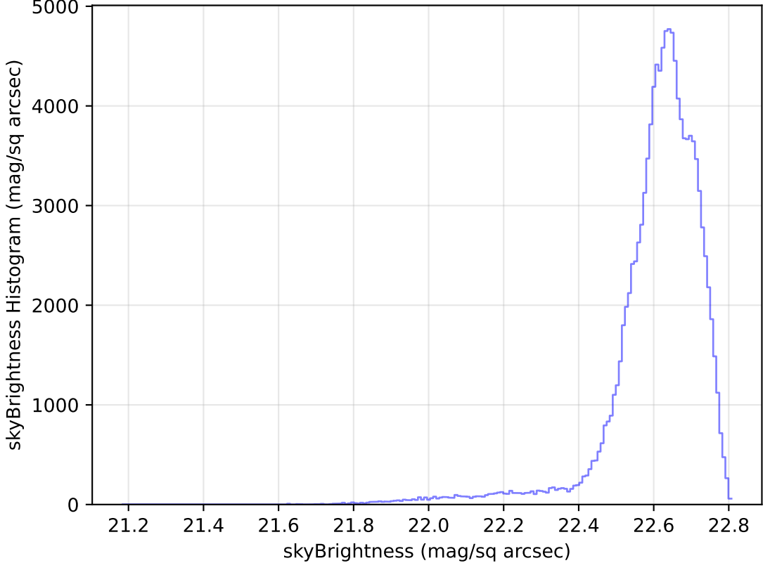
too_elab_r256_d2_gz_v3.4_10yrs All sky u band: skyBrightness Histogram
