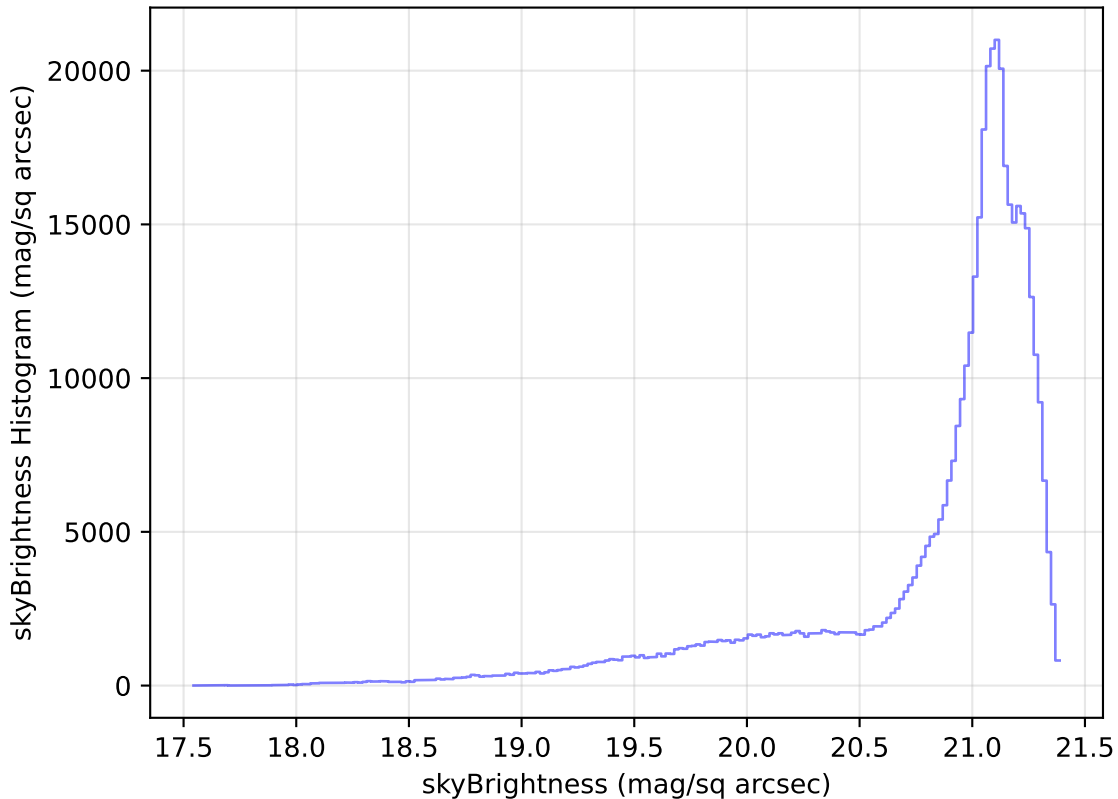
too_elab_r256_d2_gz_v3.4_10yrs All sky r band: skyBrightness Histogram
