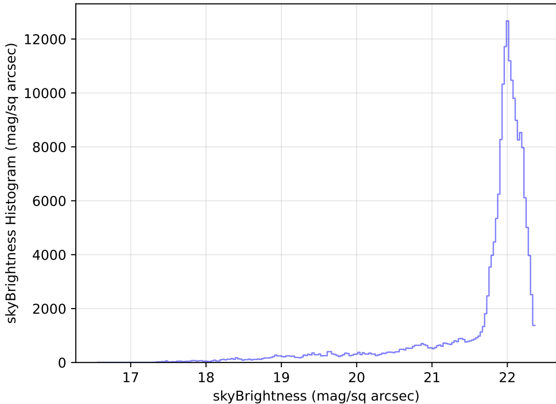
too_elab_r256_d2_gz_v3.4_10yrs All sky g band: skyBrightness Histogram
