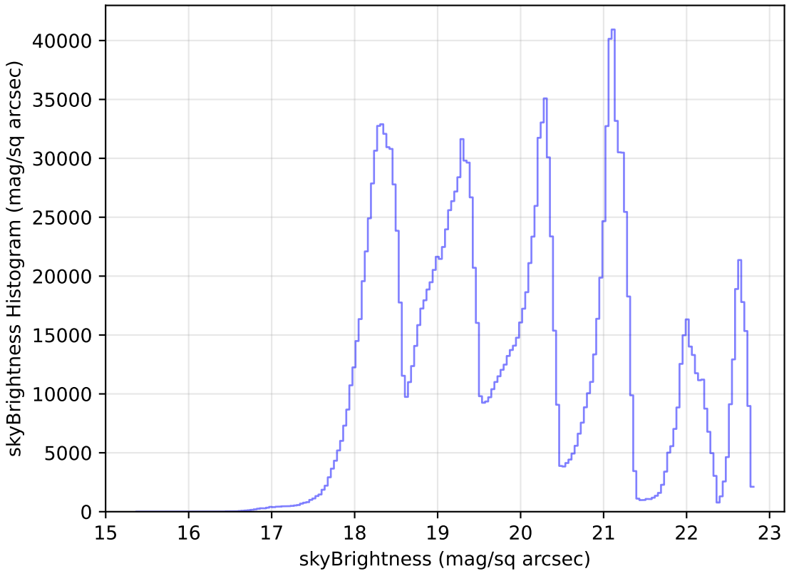
too_elab_r256_d2_gz_v3.4_10yrs All sky all bands: skyBrightness Histogram
