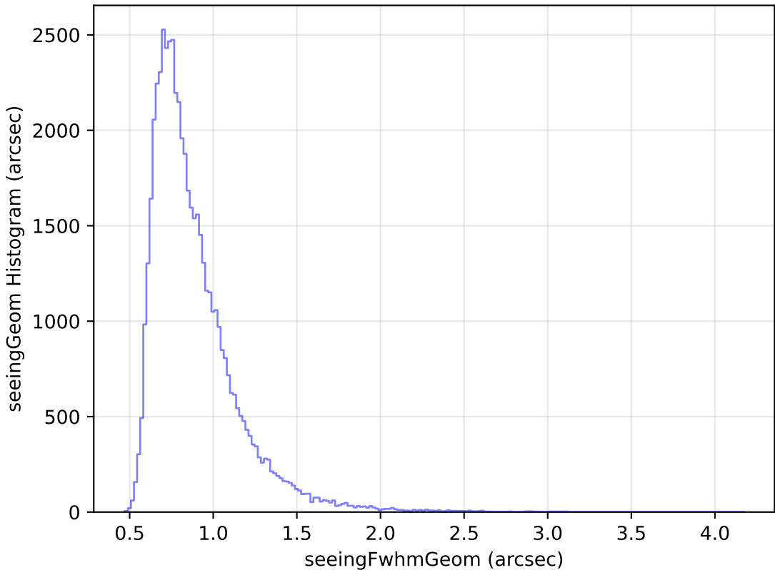
too_elab_r256_d2_gz_v3.4_10yrs Yr 1 i band: seeingGeom Histogram
