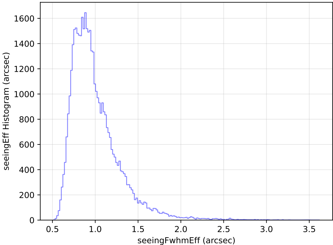
too_elab_r256_d2_gz_v3.4_10yrs Yr 1 z band: seeingEff Histogram
