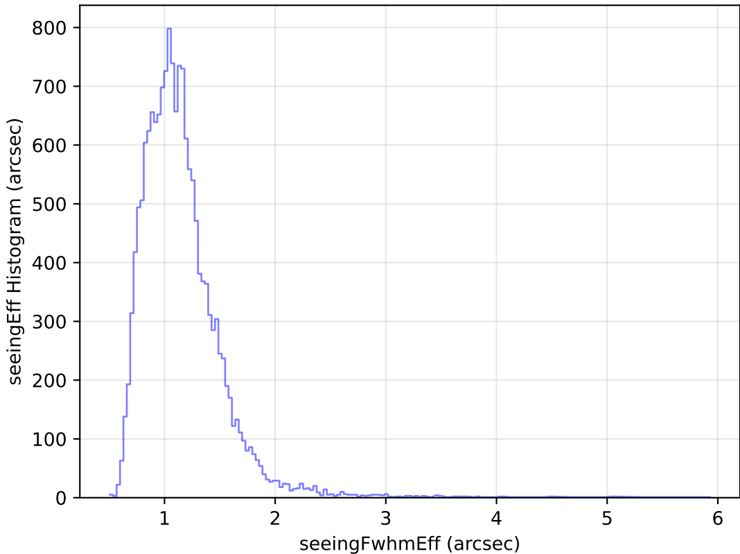
too_elab_r256_d2_gz_v3.4_10yrs Yr 1 u band: seeingEff Histogram
