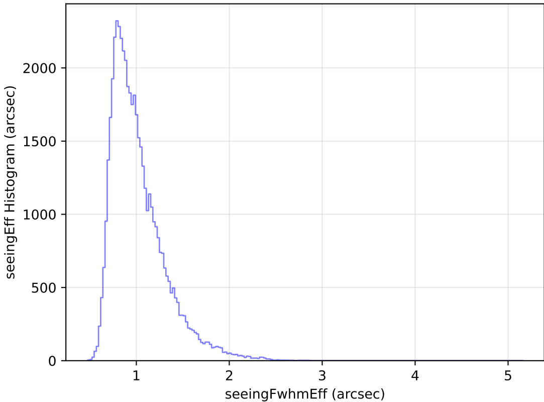
too_elab_r256_d2_gz_v3.4_10yrs Yr 1 r band: seeingEff Histogram
