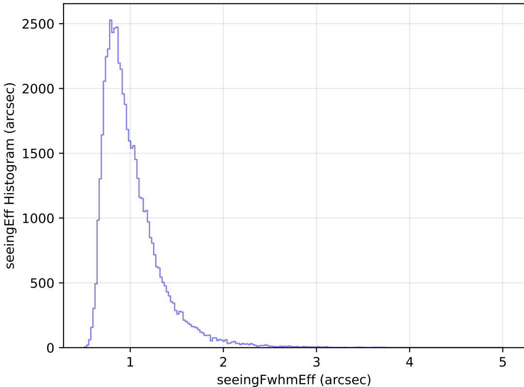
too_elab_r256_d2_gz_v3.4_10yrs Yr 1 i band: seeingEff Histogram
