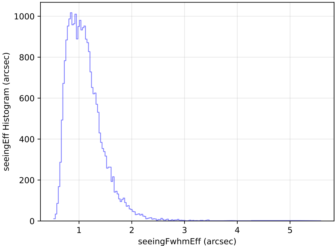
too_elab_r256_d2_gz_v3.4_10yrs Yr 1 g band: seeingEff Histogram
