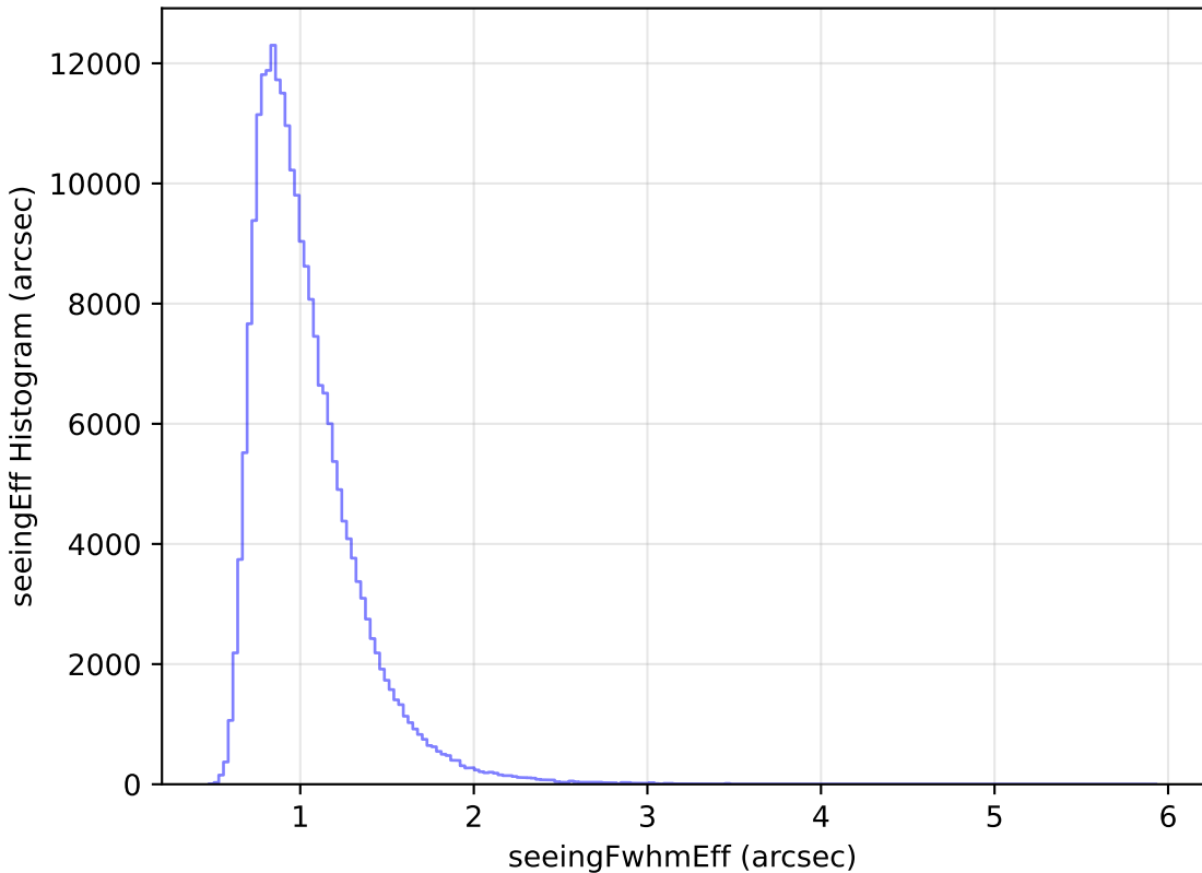
too_elab_r256_d2_gz_v3.4_10yrs Yr 1 all bands: seeingEff Histogram
