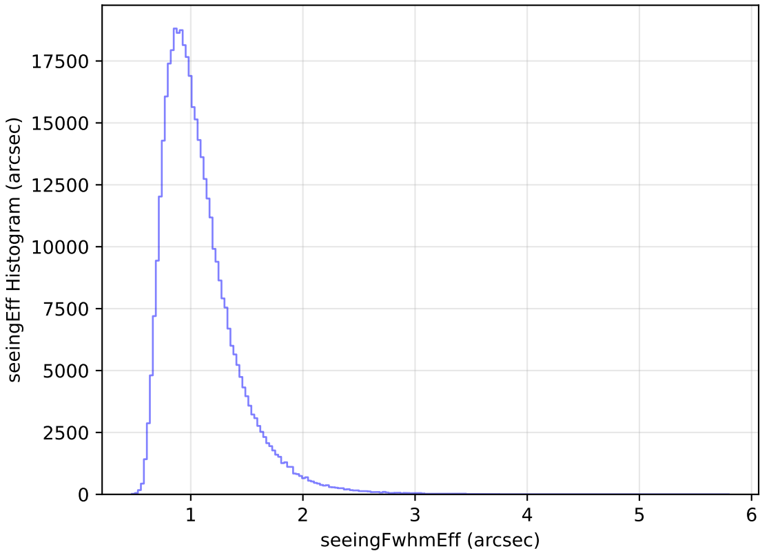
too_elab_r256_d2_gz_v3.4_10yrs WFD z band: seeingEff Histogram
