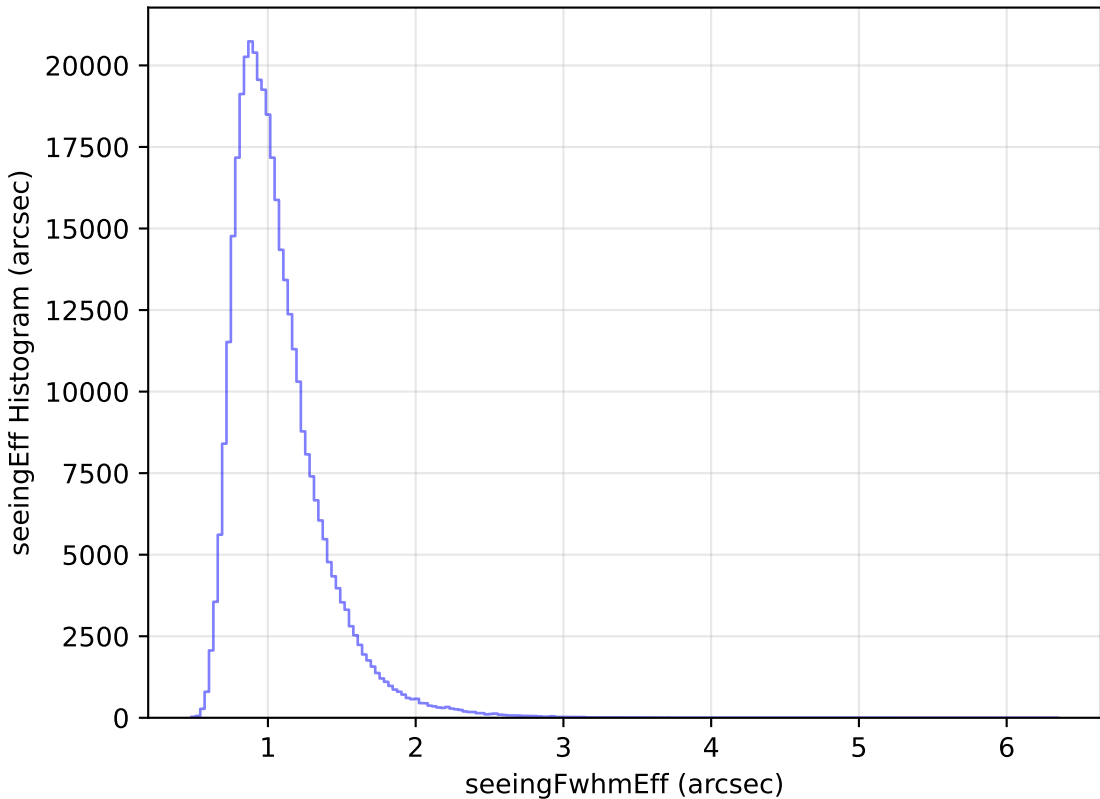
too_elab_r256_d2_gz_v3.4_10yrs WFD y band: seeingEff Histogram
