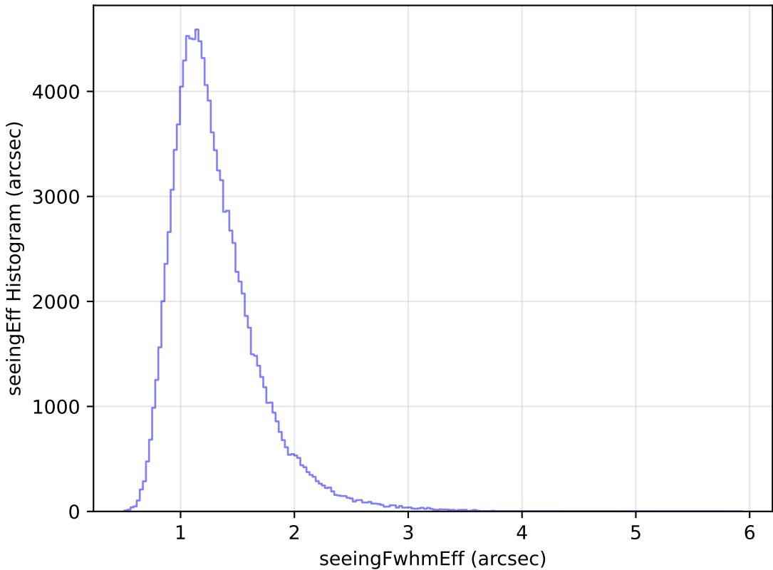
too_elab_r256_d2_gz_v3.4_10yrs WFD u band: seeingEff Histogram
