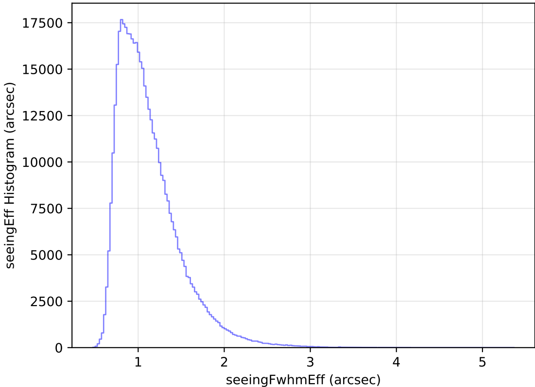
too_elab_r256_d2_gz_v3.4_10yrs WFD r band: seeingEff Histogram
