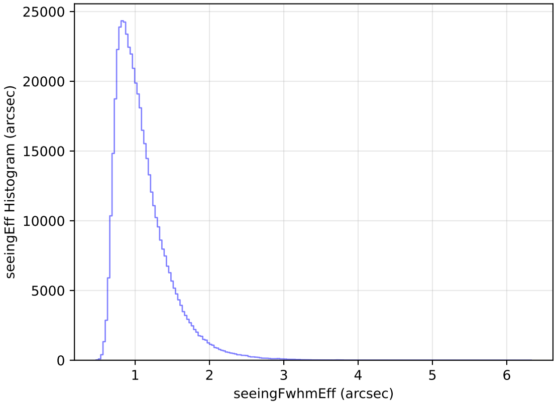
too_elab_r256_d2_gz_v3.4_10yrs WFD i band: seeingEff Histogram
