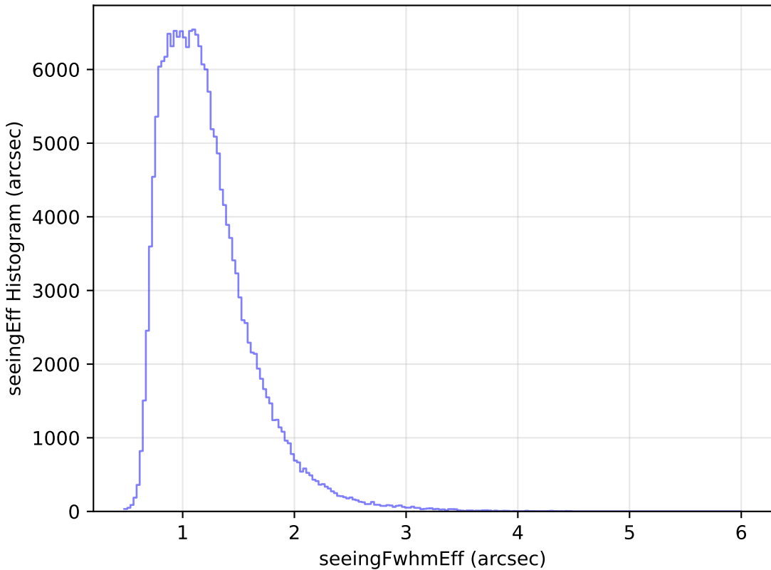
too_elab_r256_d2_gz_v3.4_10yrs WFD g band: seeingEff Histogram
