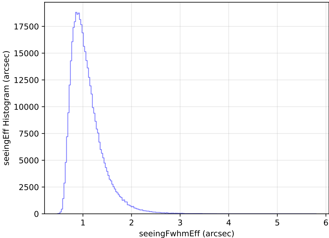
too_elab_r256_d2_gz_v3.4_10yrs All sky z band: seeingEff Histogram
