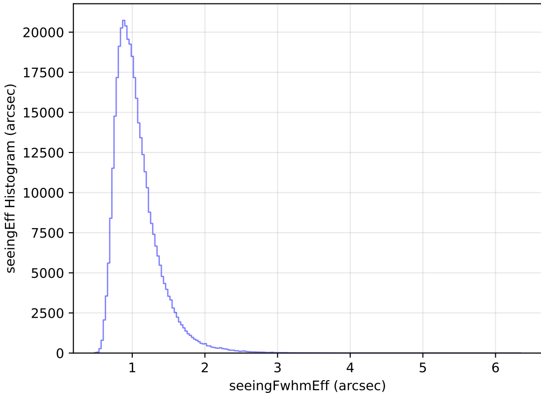
too_elab_r256_d2_gz_v3.4_10yrs All sky y band: seeingEff Histogram
