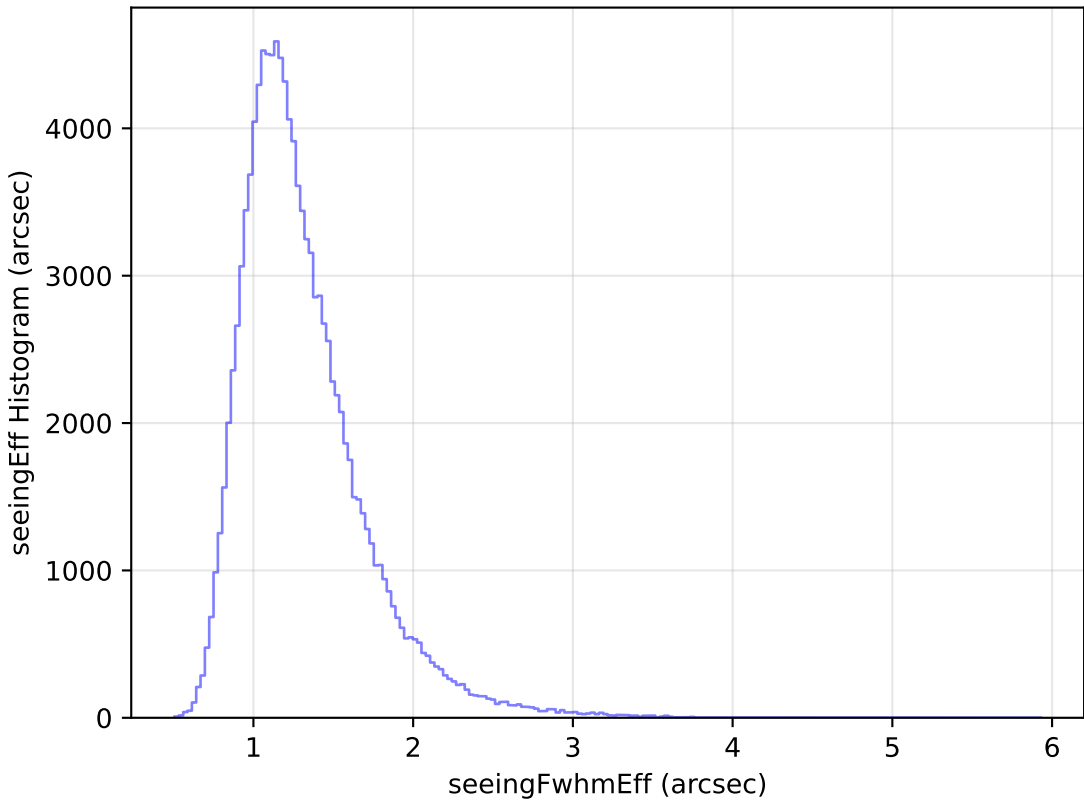
too_elab_r256_d2_gz_v3.4_10yrs All sky u band: seeingEff Histogram
