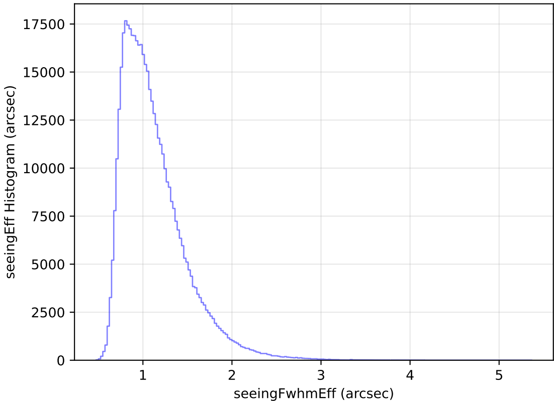
too_elab_r256_d2_gz_v3.4_10yrs All sky r band: seeingEff Histogram
