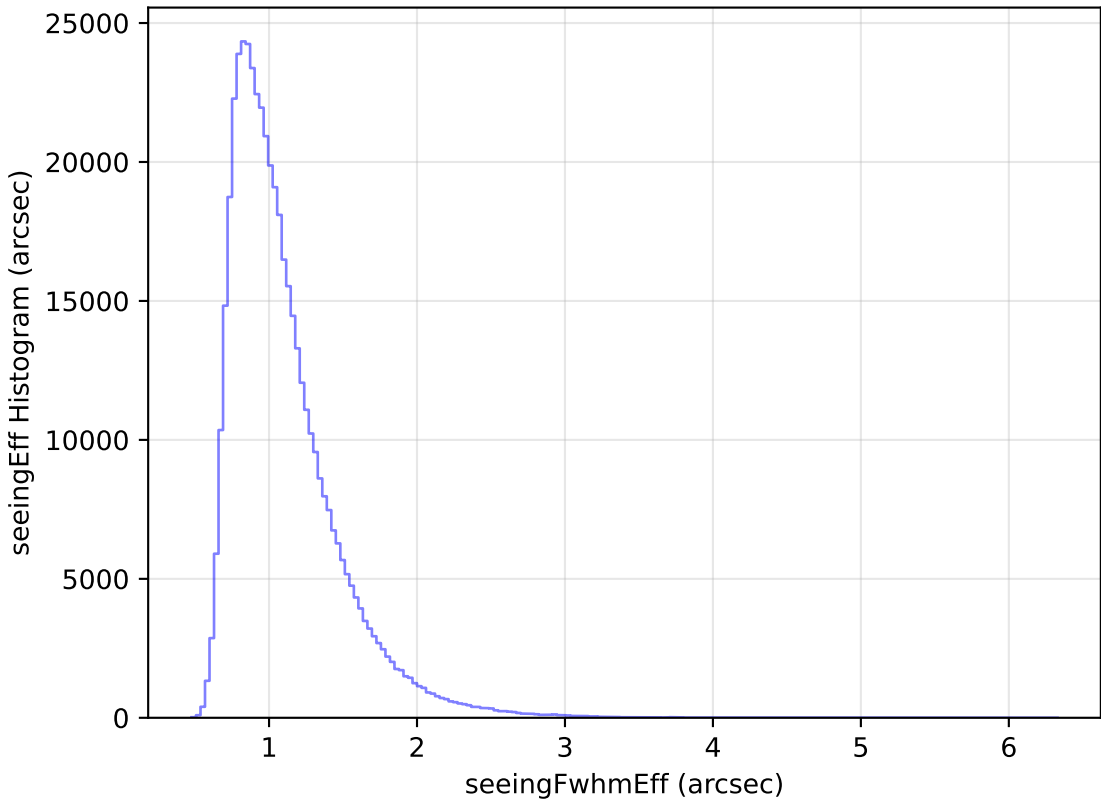
too_elab_r256_d2_gz_v3.4_10yrs All sky i band: seeingEff Histogram
