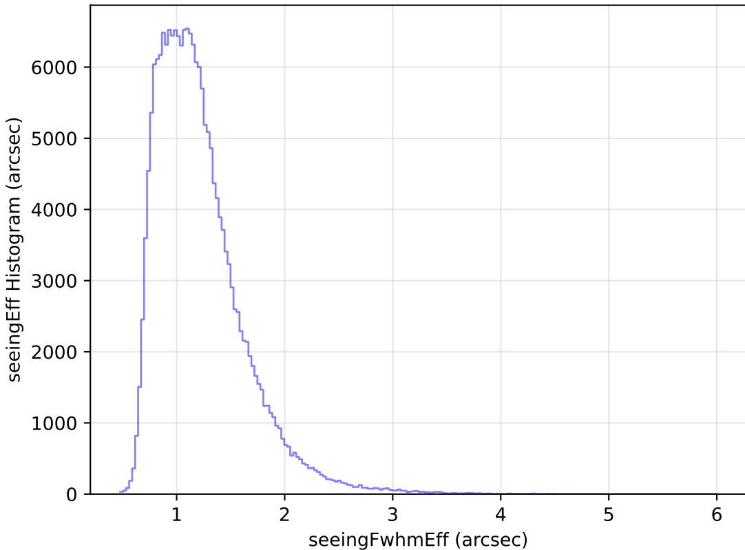
too_elab_r256_d2_gz_v3.4_10yrs All sky g band: seeingEff Histogram
