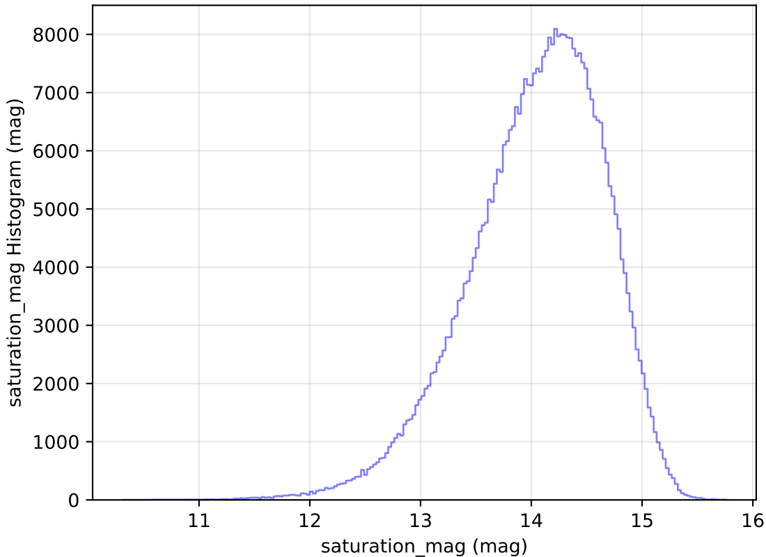
too_elab_r256_d2_gz_v3.4_10yrs WFD z band: saturation_mag Histogram
