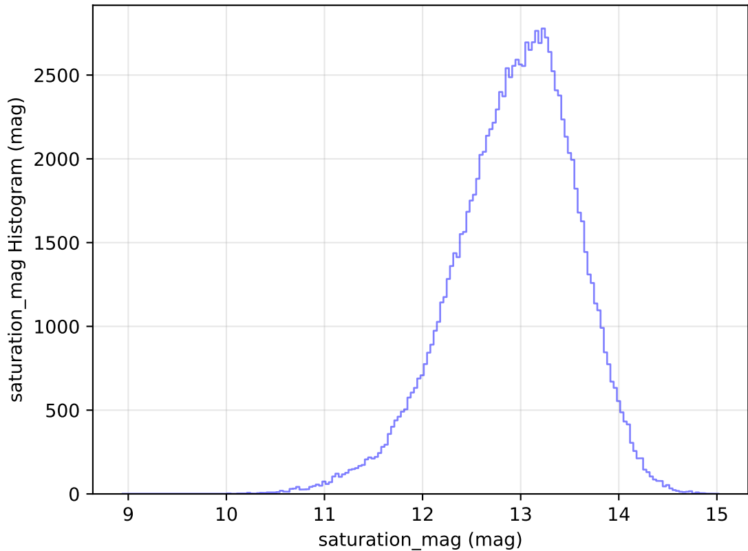
too_elab_r256_d2_gz_v3.4_10yrs WFD u band: saturation_mag Histogram
