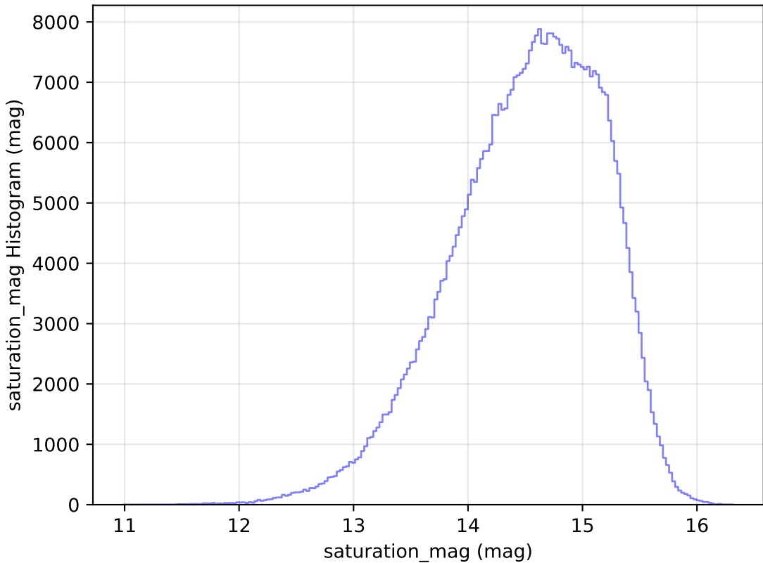
too_elab_r256_d2_gz_v3.4_10yrs WFD r band: saturation_mag Histogram
