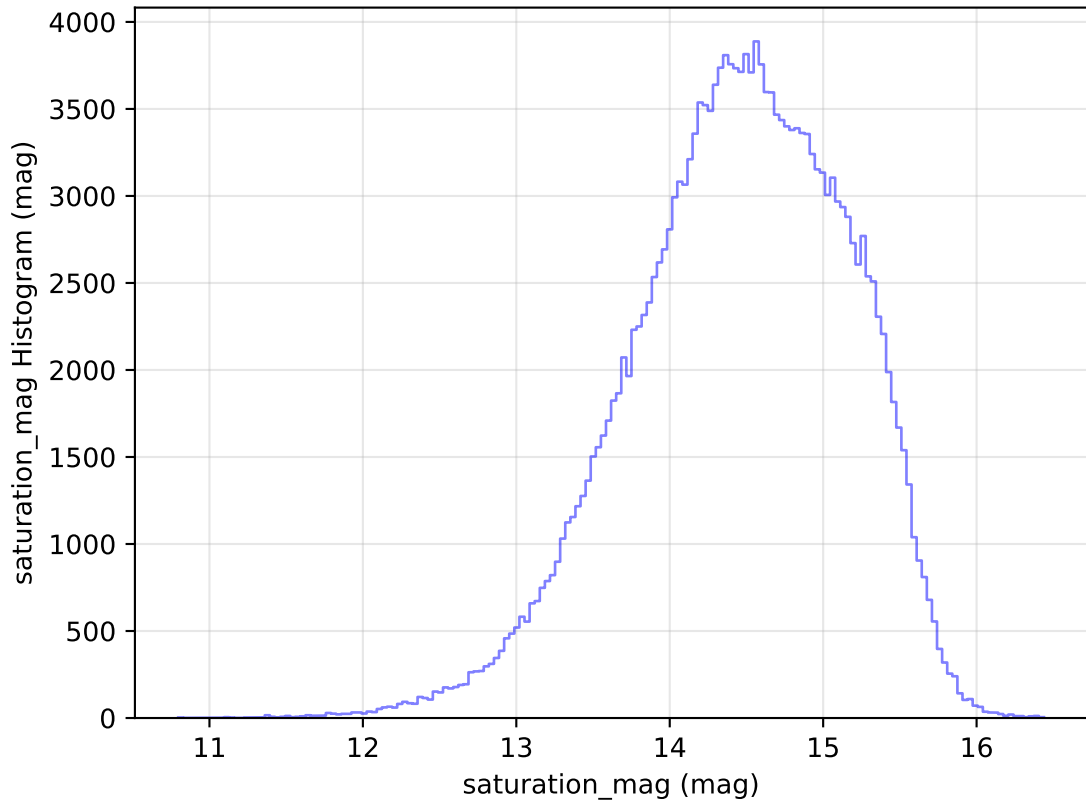
too_elab_r256_d2_gz_v3.4_10yrs WFD g band: saturation_mag Histogram
