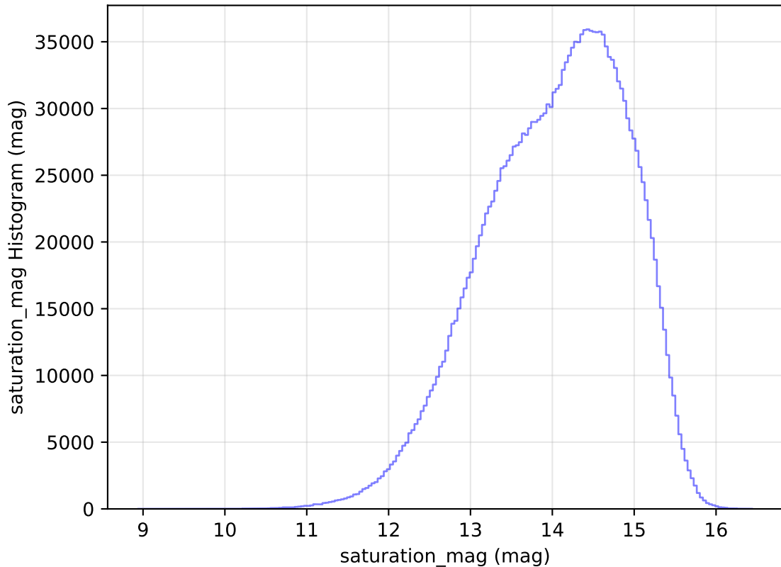
too_elab_r256_d2_gz_v3.4_10yrs WFD all bands: saturation_mag Histogram
