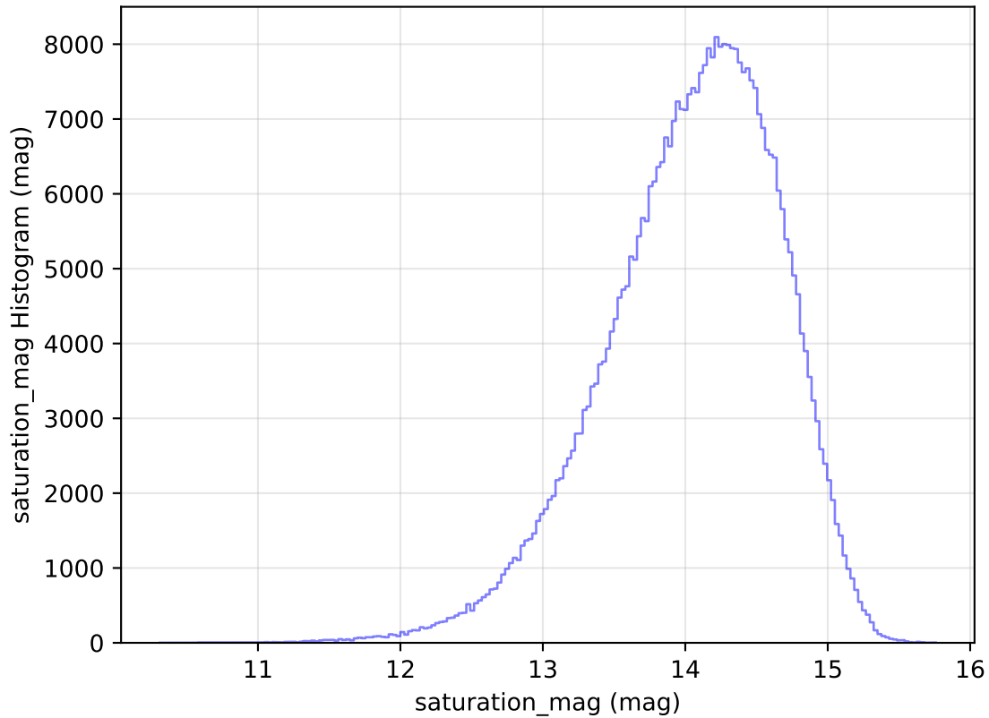
too_elab_r256_d2_gz_v3.4_10yrs All sky z band: saturation_mag Histogram
