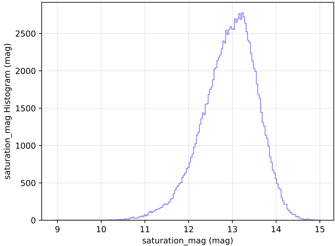
too_elab_r256_d2_gz_v3.4_10yrs All sky u band: saturation_mag Histogram
