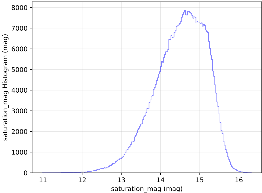
too_elab_r256_d2_gz_v3.4_10yrs All sky r band: saturation_mag Histogram
