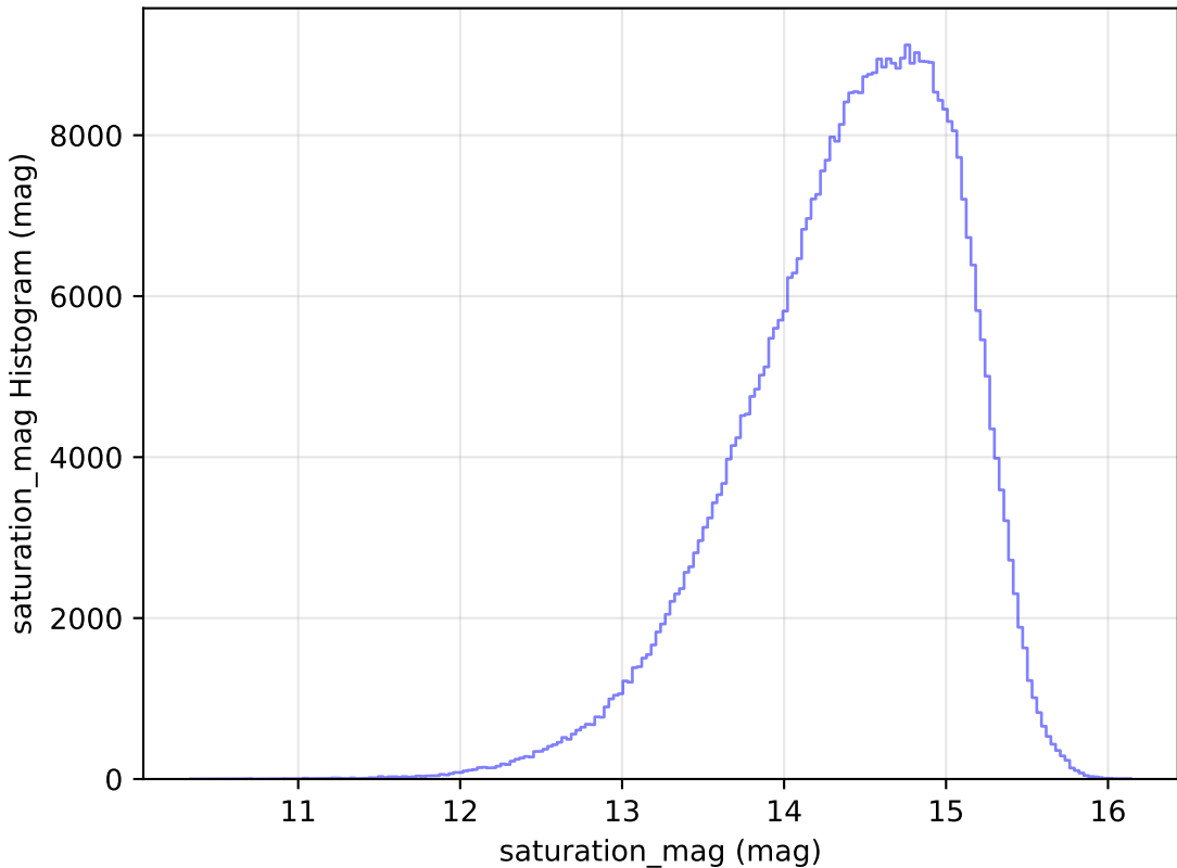
too_elab_r256_d2_gz_v3.4_10yrs All sky i band: saturation_mag Histogram
