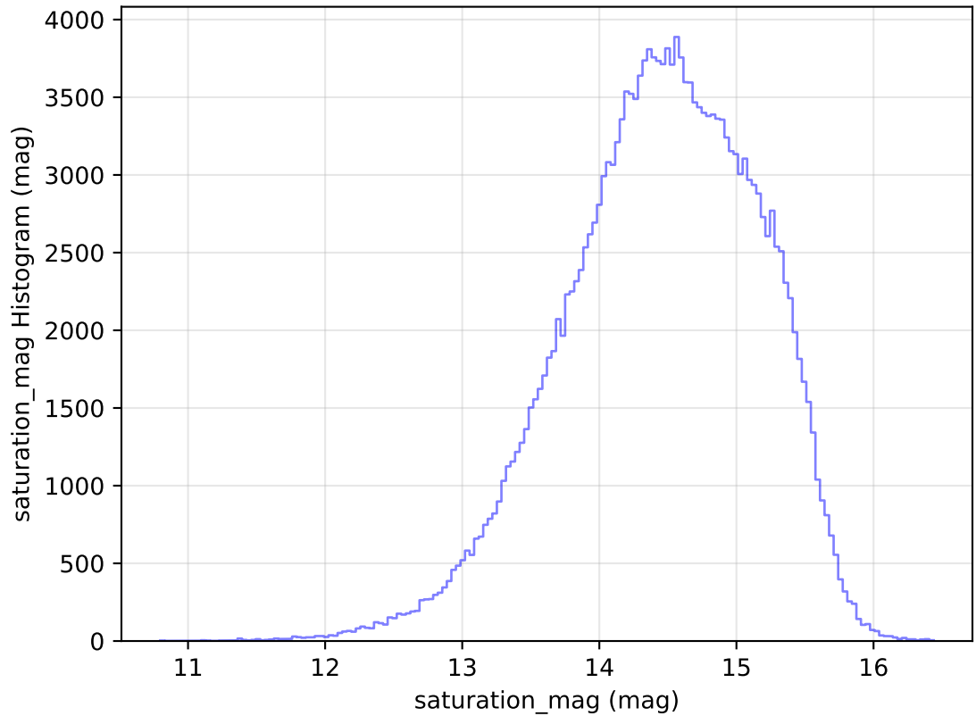
too_elab_r256_d2_gz_v3.4_10yrs All sky g band: saturation_mag Histogram
