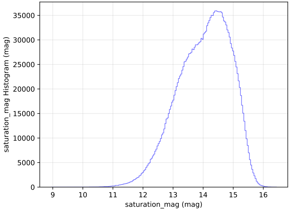
too_elab_r256_d2_gz_v3.4_10yrs All sky all bands: saturation_mag Histogram
