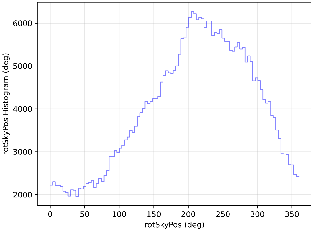
too_elab_r256_d2_gz_v3.4_10yrs WFD y band: rotSkyPos Histogram
