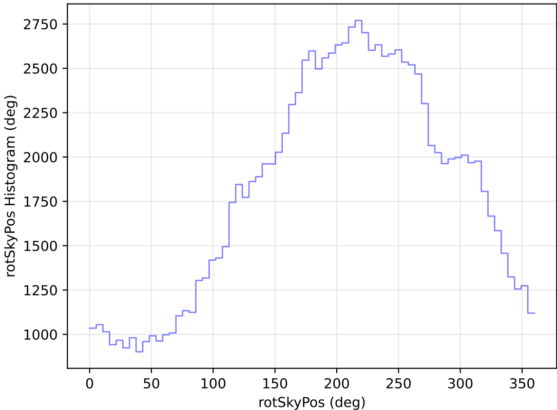
too_elab_r256_d2_gz_v3.4_10yrs WFD u band: rotSkyPos Histogram
