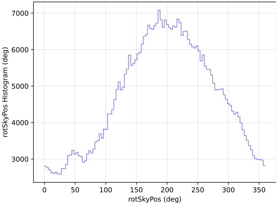
too_elab_r256_d2_gz_v3.4_10yrs WFD r band: rotSkyPos Histogram
