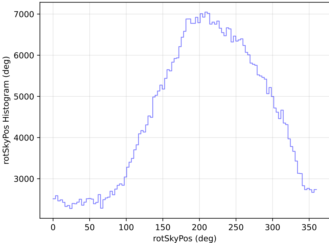
too_elab_r256_d2_gz_v3.4_10yrs WFD i band: rotSkyPos Histogram
