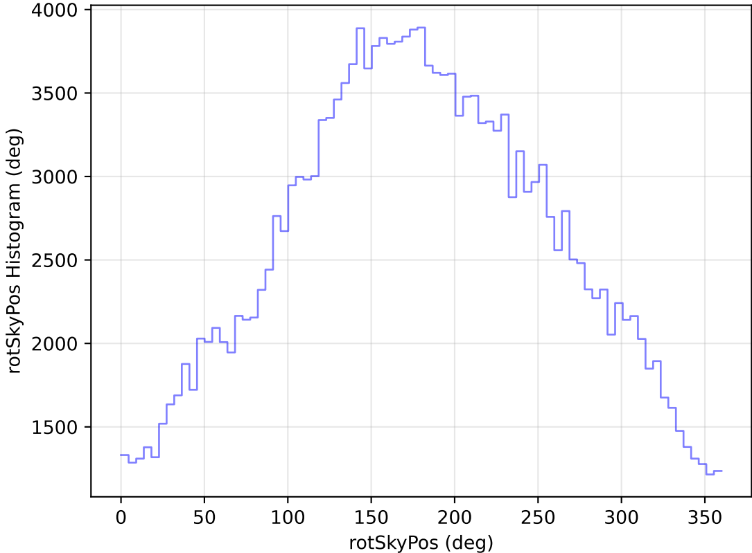
too_elab_r256_d2_gz_v3.4_10yrs WFD g band: rotSkyPos Histogram
