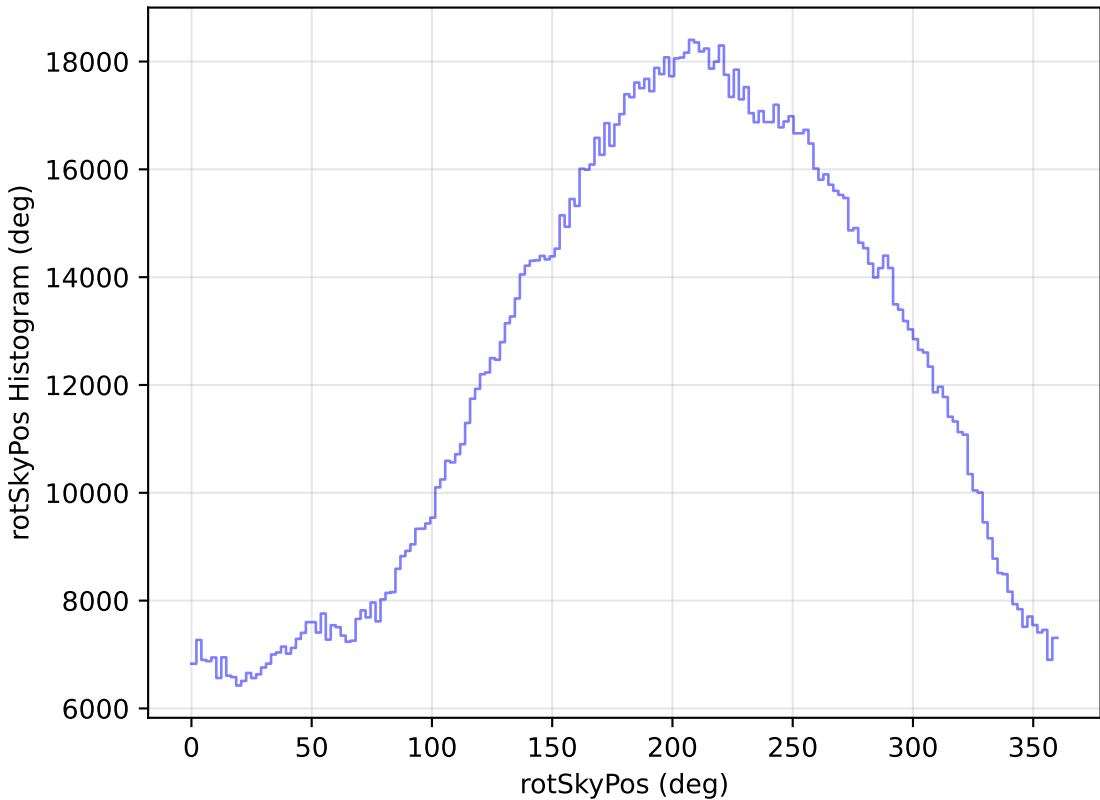
too_elab_r256_d2_gz_v3.4_10yrs WFD all bands: rotSkyPos Histogram
