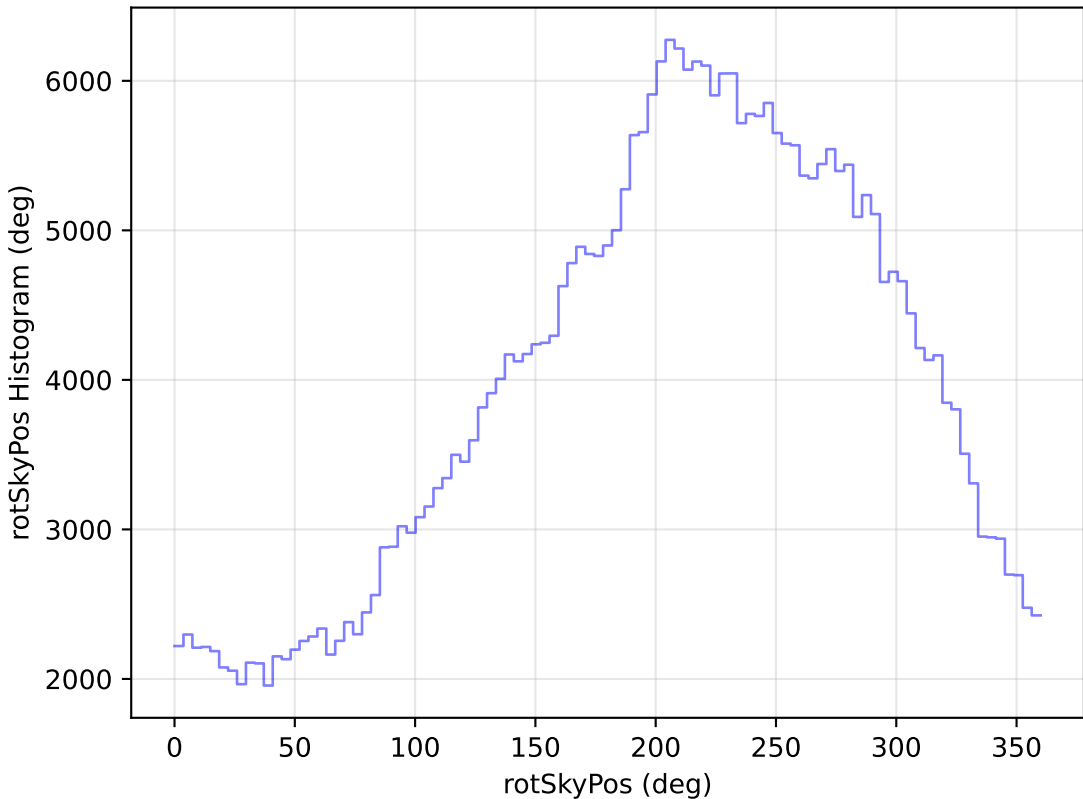
too_elab_r256_d2_gz_v3.4_10yrs All sky y band: rotSkyPos Histogram
