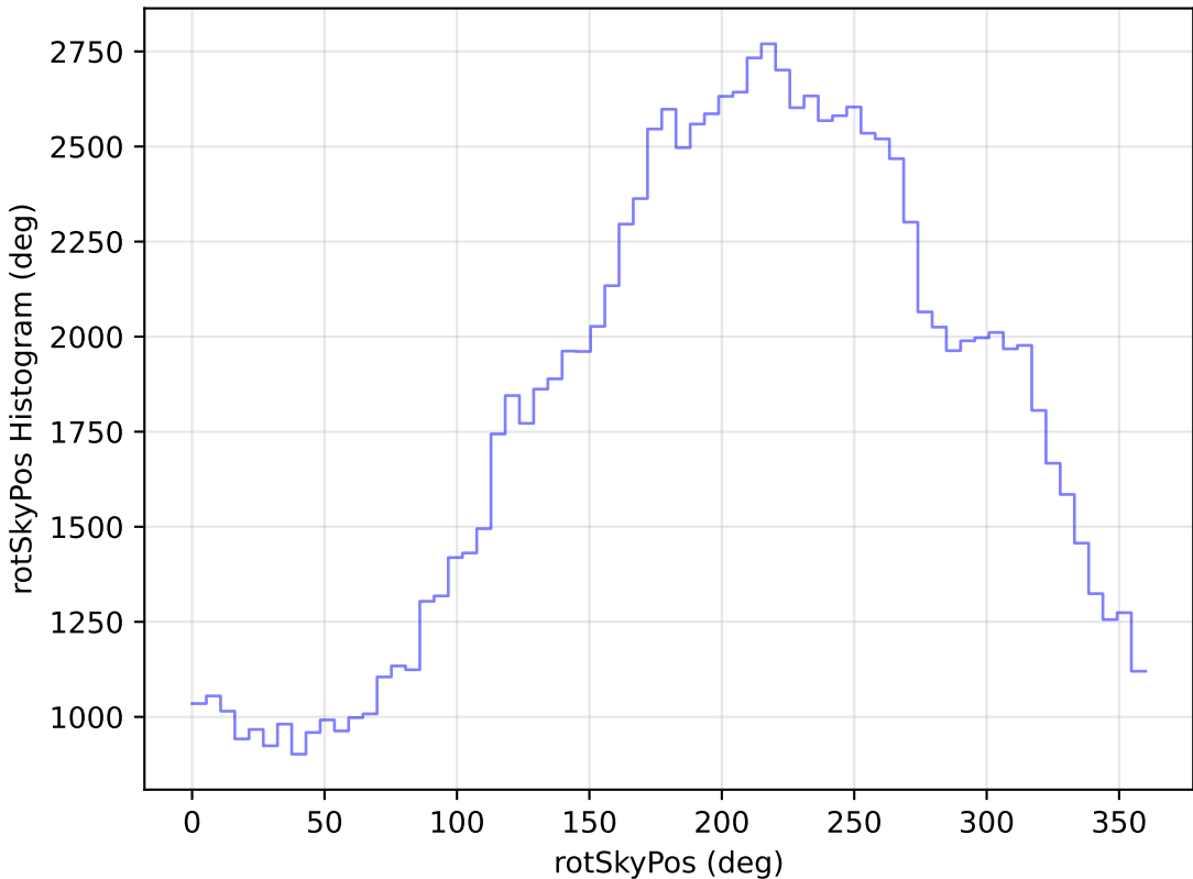
too_elab_r256_d2_gz_v3.4_10yrs All sky u band: rotSkyPos Histogram
