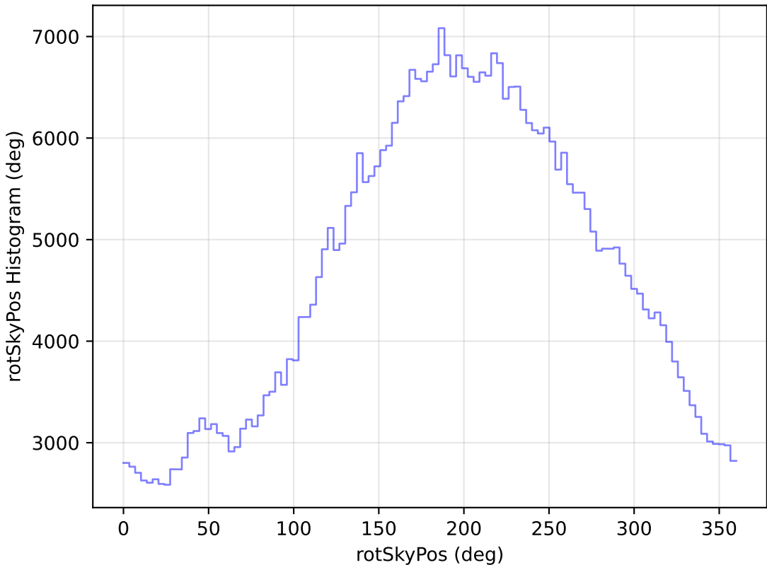
too_elab_r256_d2_gz_v3.4_10yrs All sky r band: rotSkyPos Histogram
