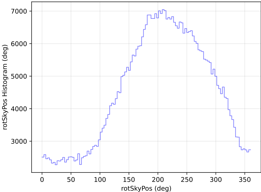
too_elab_r256_d2_gz_v3.4_10yrs All sky i band: rotSkyPos Histogram
