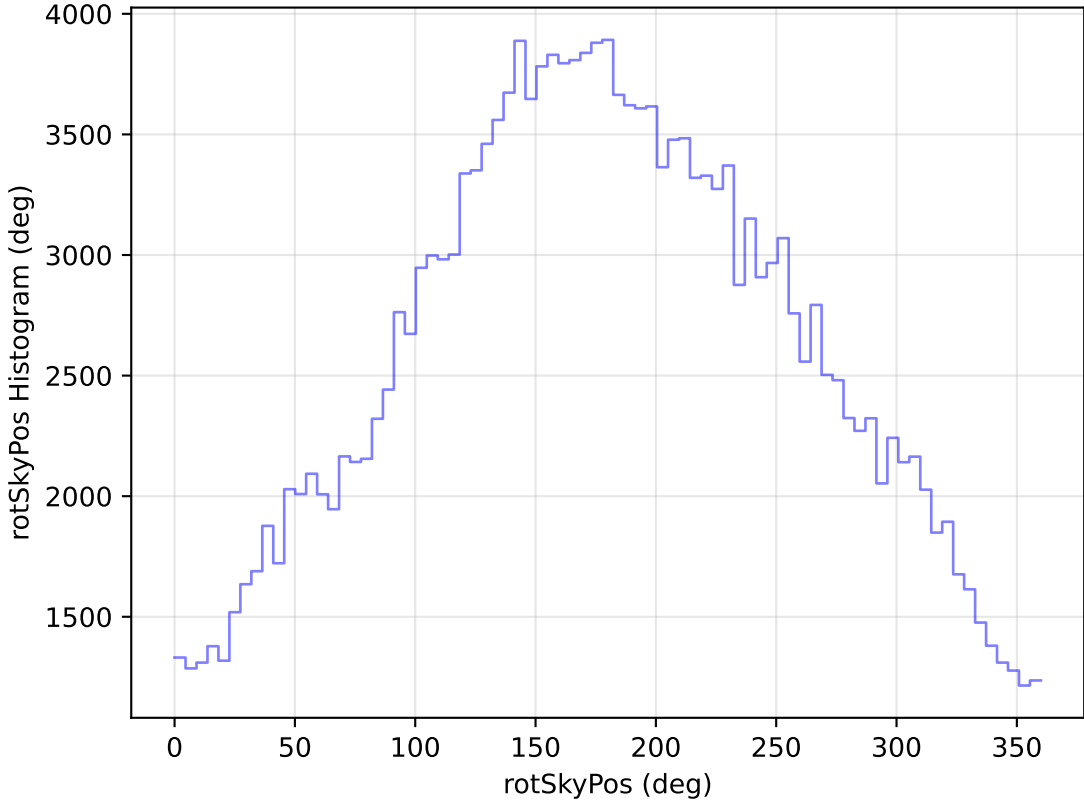
too_elab_r256_d2_gz_v3.4_10yrs All sky g band: rotSkyPos Histogram
