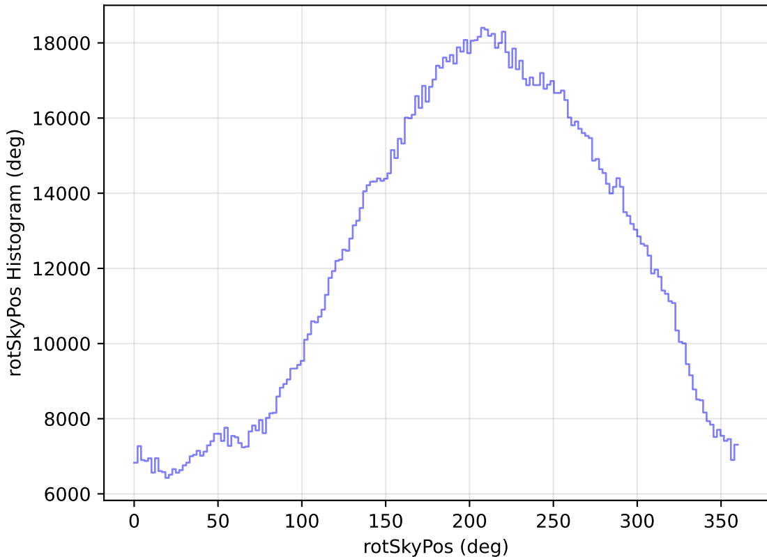
too_elab_r256_d2_gz_v3.4_10yrs All sky all bands: rotSkyPos Histogram
